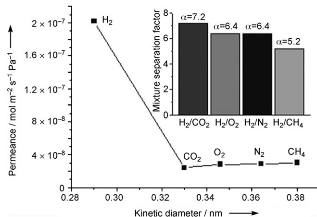
Figure 3. Single-gas permeances of different gases on the ZIF-22 membrane at 323 K as a function of the kinetic diameter. The inset shows the mixture separation factor for \text{H}_2 over other gases, determined by gas chromatography.
